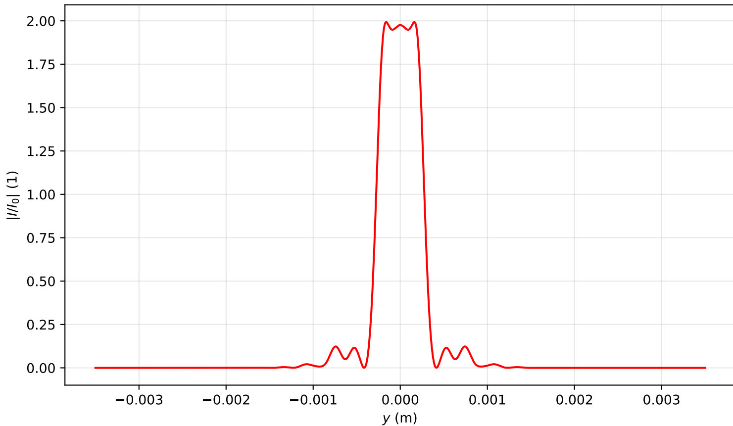
Intensity profile I(x=0, y, z=0.716)/I_0 , P_{in}=7.5P_{cr} , artificial time
